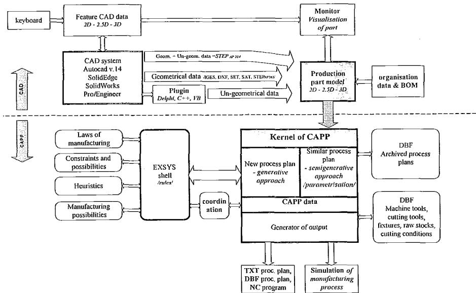
Fig. 8. The basic conception of CAD/CAPP system
