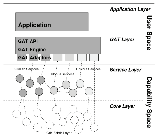
Fig. 1. The GAT framework software architecture
